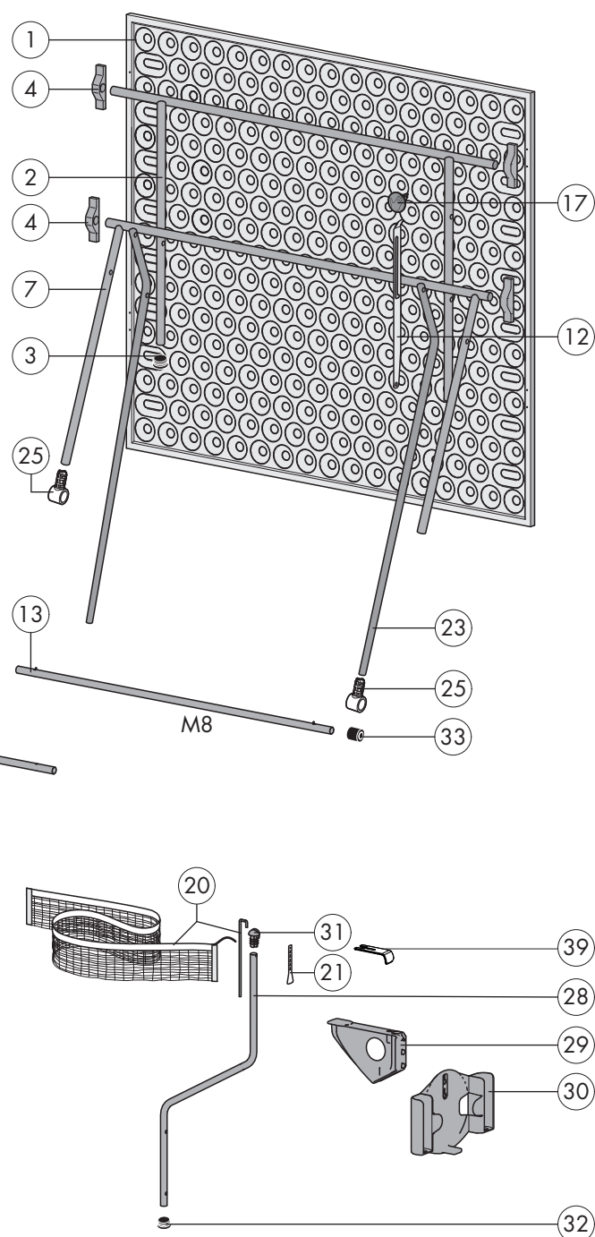
MATCH 3.0 07175-600 outdoor
