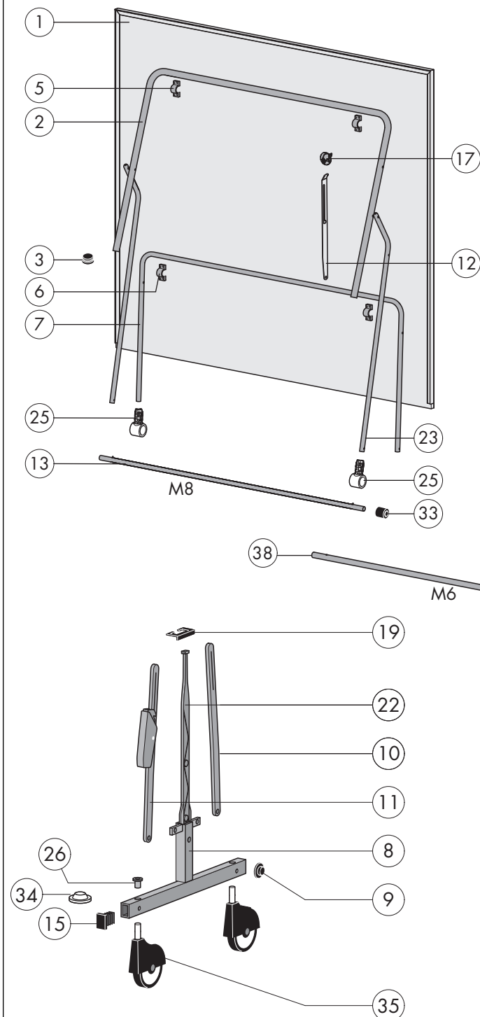
MATCH 3.0 07135-600 indoor
